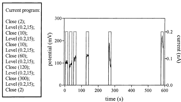
Fig. 8. Chronopotentiometric curves for bilayer lipid membrane registered under programmable current with changeable interruptions for a short circuit of the electrodes for an increasing period of time. Solid line, left axis, potential changes; dashed line, right axis, current changes. Sequence of registration: 0.2 nA current flowing within 15 s, interruption for a short circuit of the current electrodes. The time of interruption increases in consecutive repetitions. The frame on the left side of the figure contains the parameters of the current program. Forming solution: phosphatidylcholine/cholesterol (7:3 w/w). Electrolyte: 0.1 M KCl, HEPES pH 7.0.
